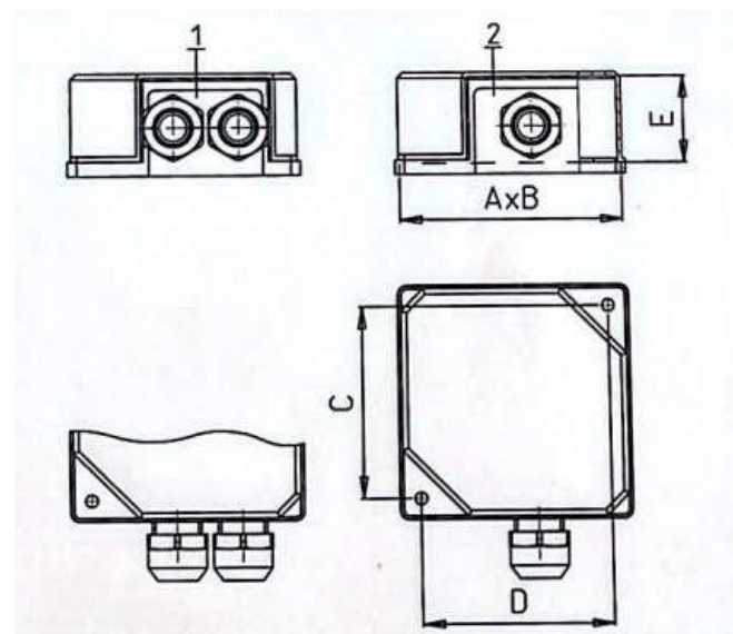
CPVPS Drawing
