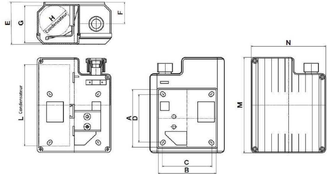
FMAG CC80-112 drawing
