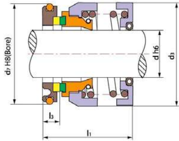
PXB Drawing
