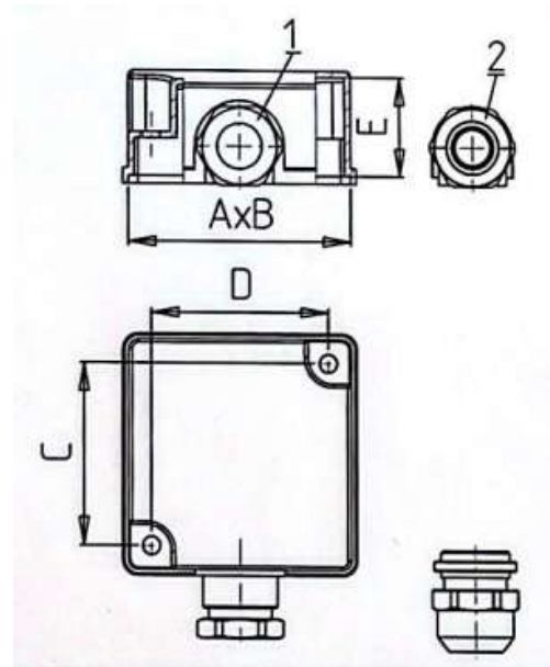
CPF Drawing
