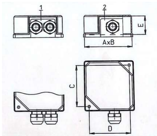
CPV Drawing
